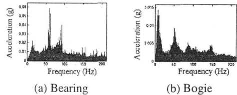
Fig. 2 FFT Analysis of Vibration
