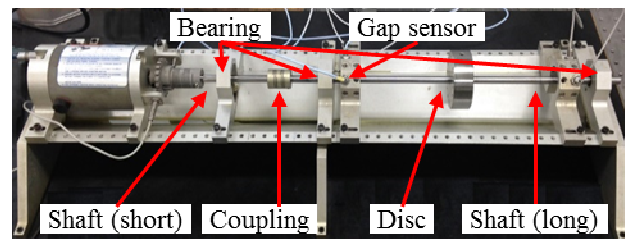
Fig. 2 RK4 Test-bed
